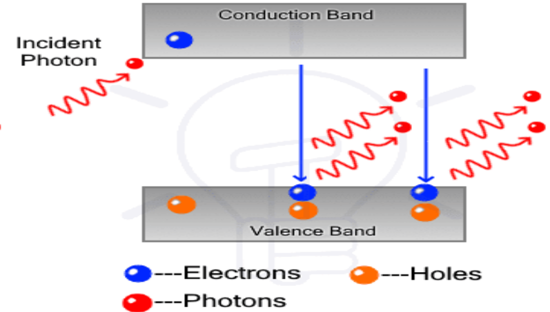
Stimulated Emission
