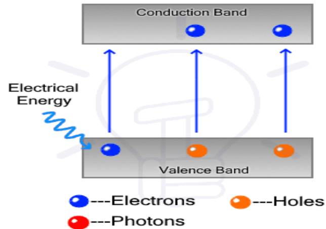
Energy Absorption
