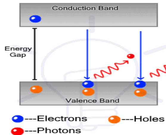
Spontaneous Emission
